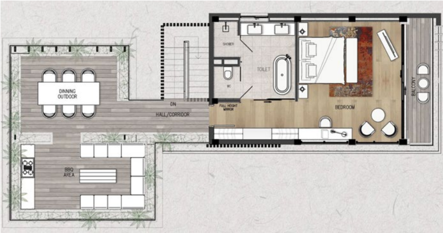
Second Floor
